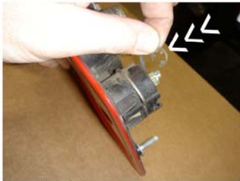
Before the bucket comes out of the door, remove the "C" clip to remove the Lock Rod Actuator
