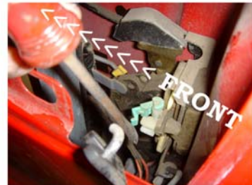
The clip unsnaps from the outside edge, towards the front
